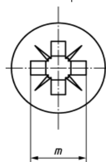
impronta croce Forma Z cross recess Form Z
